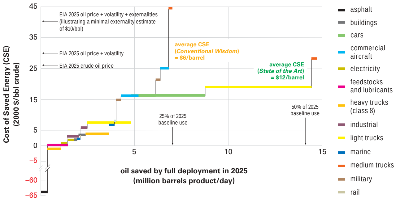
Figure 28: Supply curve summarizing Conventional Wisdom and State of the Art technologies for efficient use of oil, analyzed on pp. 43–99 above, hypothetically assuming full implementation in 2025. We assume EIA's convention of expressing savings volume in Mbb/d of product delivered to end users, totaling 28.3 Mbb/d in 2025. On the y-axis we use a value-chain adjustment for wholesale and retail products to normalize CSE to $/bbl crude. This method (pp. 40–41) accounts for differences in production and delivery costs of different products as well as energy content contained. The total State of the Art efficiency potential could save more than half of projected 2025 oil use at an average cost less than half of EIA's projected 2025 crude-oil price. Realistic implementation fractions, rates, and methods for efficient end-use will be discussed starting on p.169 below, and additional oil-saving potential from supply substitutions, starting on p. 103.
