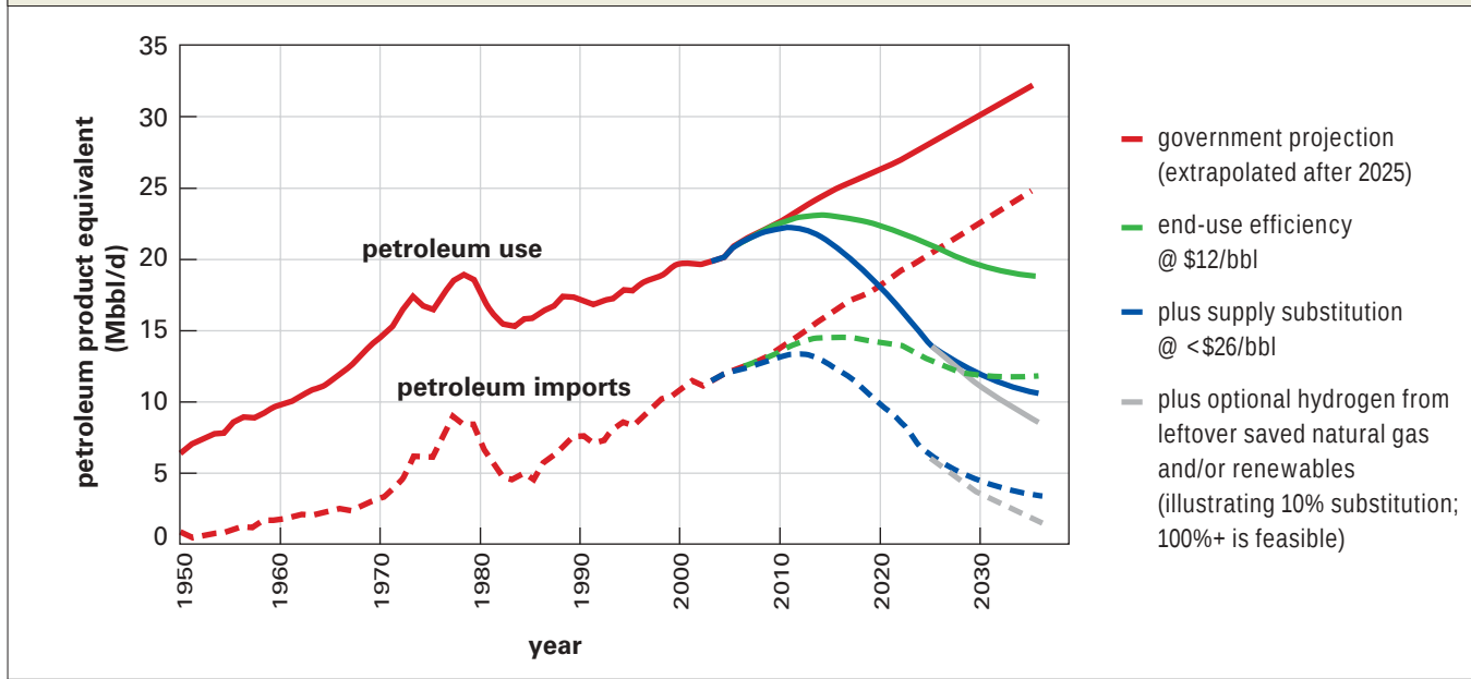
Figure 38: The path beyond oil becomes even more flexible if the hydrogen option is added As usual, the difference between petroleum use and petroleum imports is EIA's forecast of domestic petroleum production, which by law excludes all areas now off-limits. That oil output isn't adjusted here for slower depletion, which in practice would make domestic oil resources last longer or permit oil from particularly high-cost or sensitive areas to be left untouched. The gray line illustrates the first 10% stock capture of all end-uses by hydrogen over the decade starting in 2025, with far more still to come.
