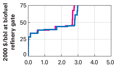
30a Conventional Wisdom biofuel supply (Mbb/d)
