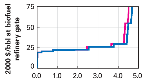
30b State of the Art biofuel supply (Mbb/d)
